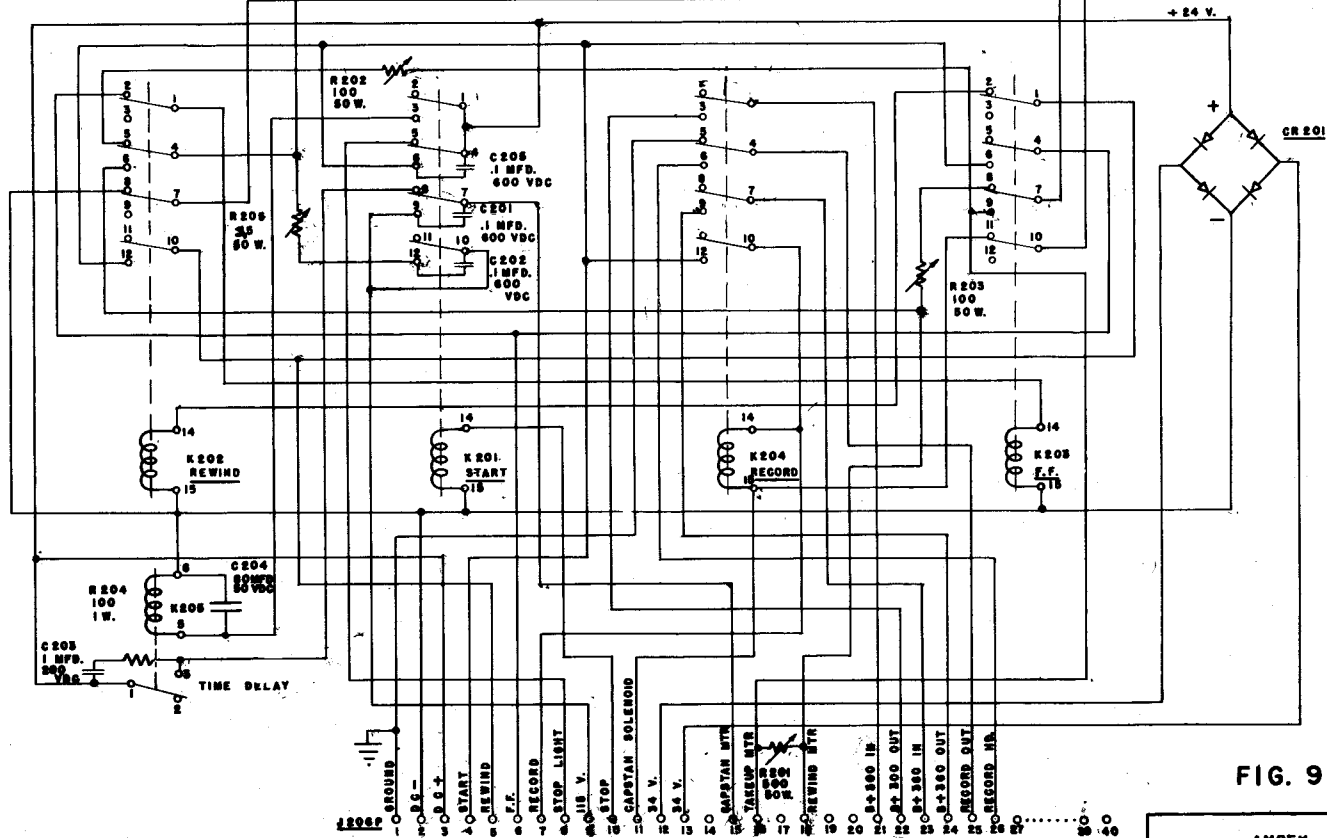
MODEL 200A - MAGNETIC TAPE RECORDER-RELAY CHASSIS SCHEMATIC DIAG.
