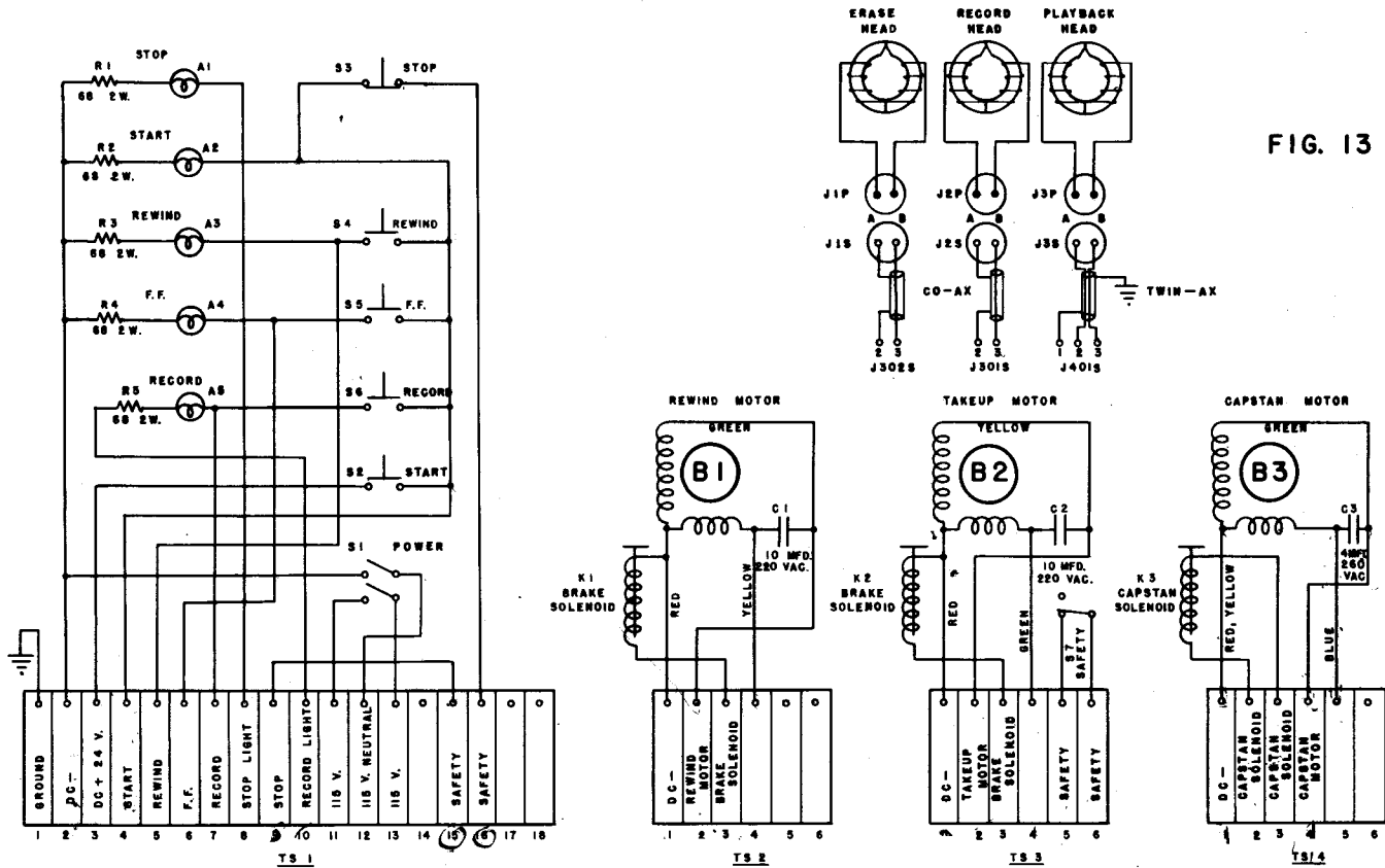
MODEL 200A - MAGNETIC TAPE RECORDER - TOP PLATE SCHEMATIC DIAG.
